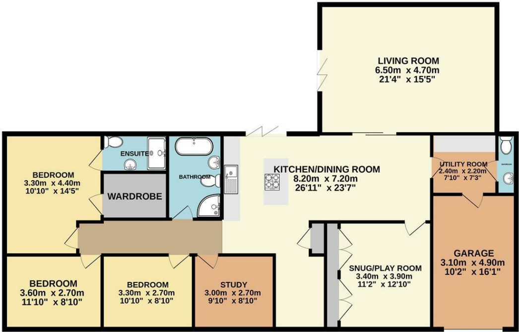
GROUND FLOOR 163.9 sq.m. (1764 sq.ft.) approx.
